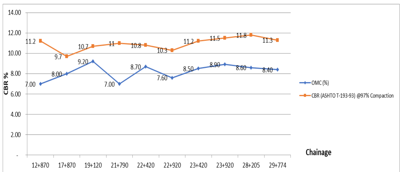
Fig. 3.2 Comparative Plot of Moisture Content & CBR at 97% MDD of Existing Subgrade Soil
